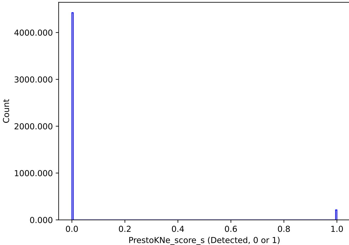
too_elab_r8_d3_ugrizy_v3.4_10yrs : PrestoKNe_score_s
