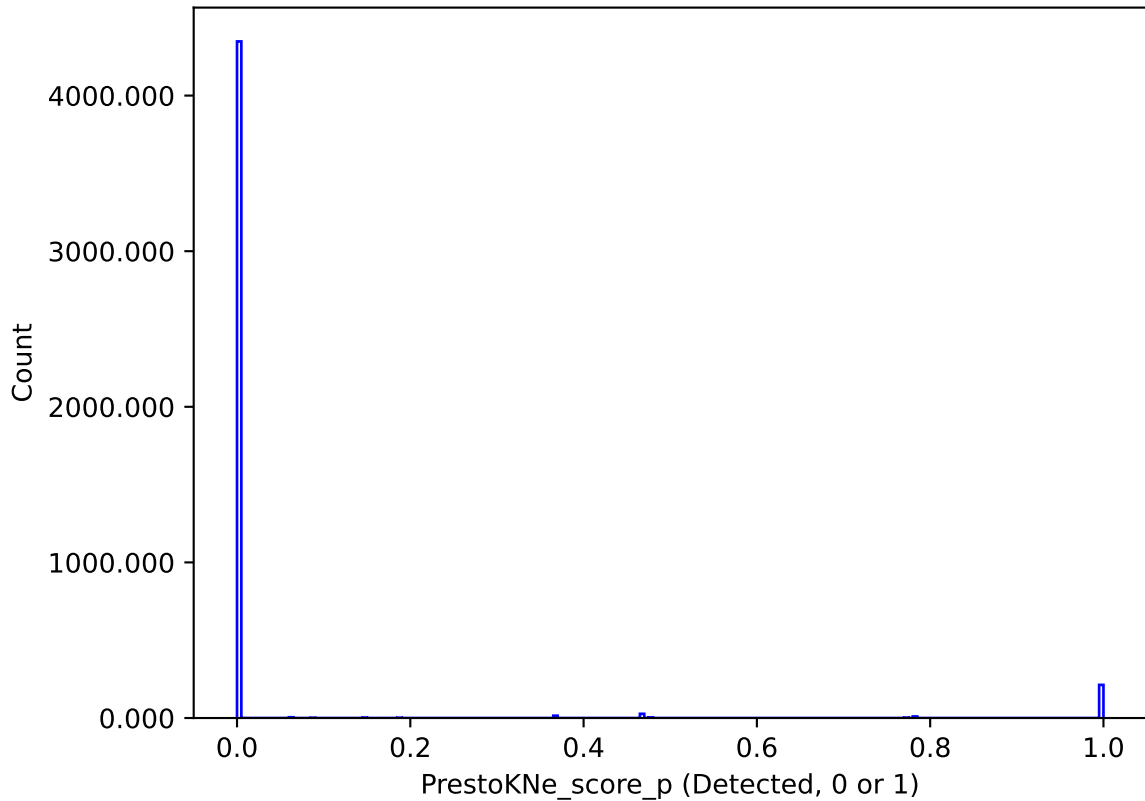
too_elab_r8_d3_ugrizy_v3.4_10yrs : PrestoKNe_score_p
