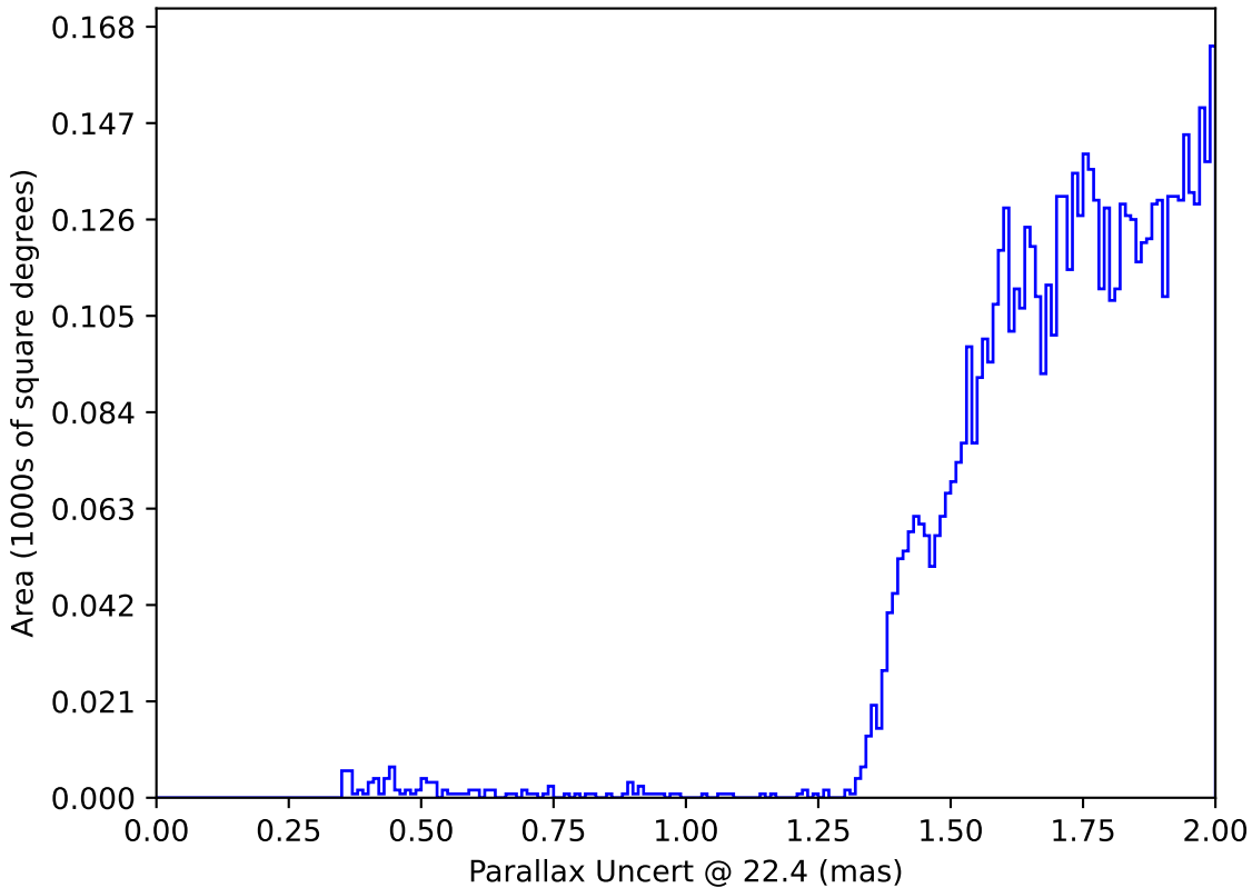
too_elab_r8_d3_ugrizy_v3.4_10yrs : Parallax Uncert @ 22.4
