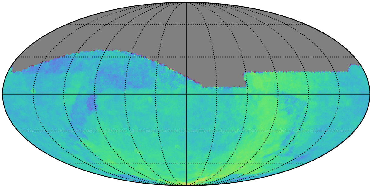
too_elab_r8_d3_ugrizy_v3.4_10yrs : Parallax Coverage @ 24.0
