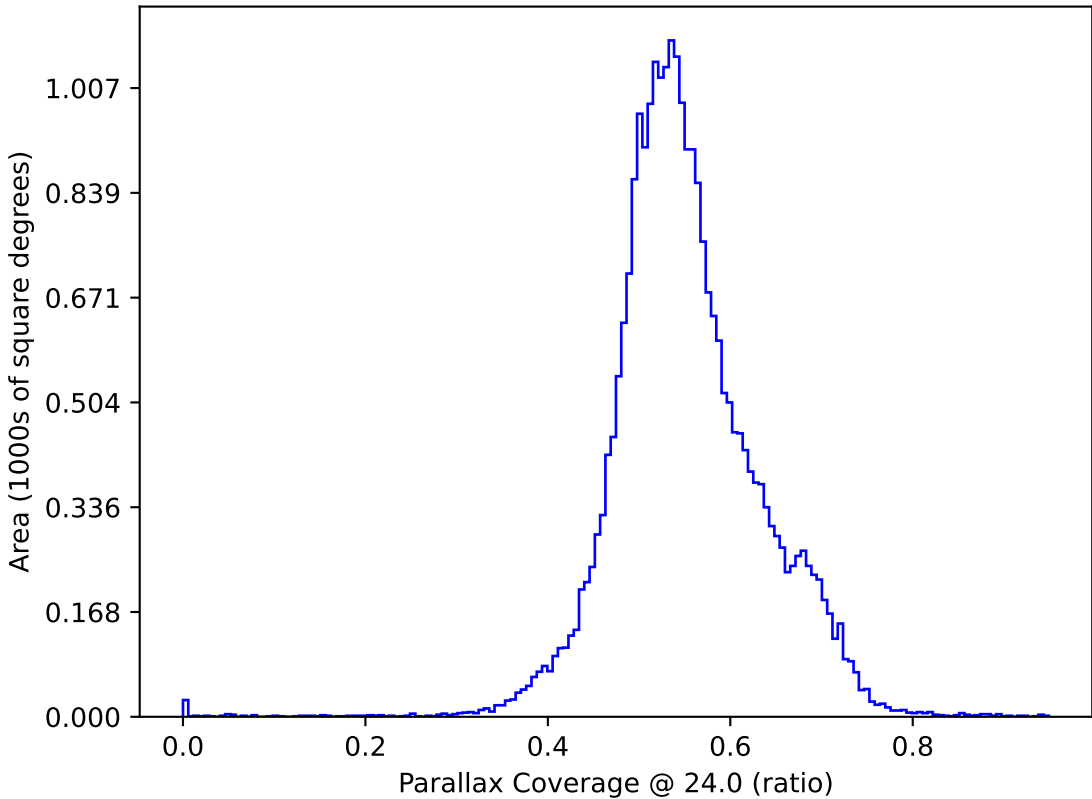
too_elab_r8_d3_ugrizy_v3.4_10yrs : Parallax Coverage @ 24.0
