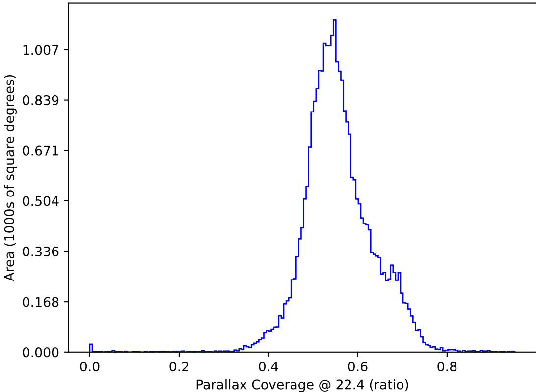
too_elab_r8_d3_ugrizy_v3.4_10yrs : Parallax Coverage @ 22.4
