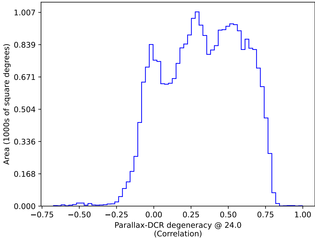
too_elab_r8_d3_ugrizy_v3.4_10yrs : Parallax-DCR degeneracy @ 24.0
