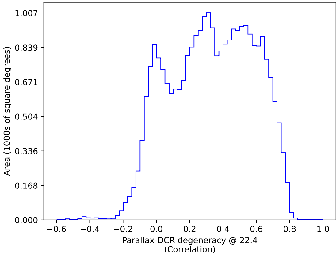
too_elab_r8_d3_ugrizy_v3.4_10yrs : Parallax-DCR degeneracy @ 22.4
