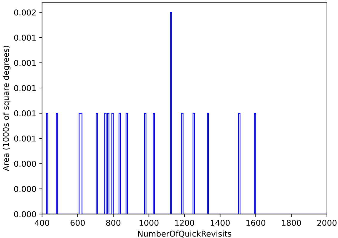
too_elab_r8_d3_ugrizy_v3.4_10yrs : NumberOfQuickRevisits
