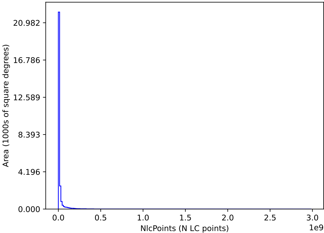
too_elab_r8_d3_ugrizy_v3.4_10yrs : NlcPoints
