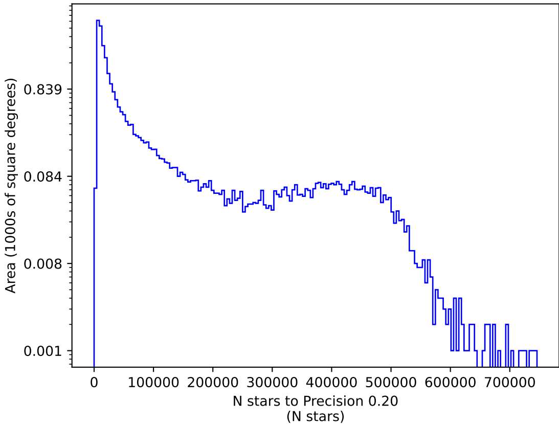
too_elab_r8_d3_ugrizy_v3.4_10yrs r: N stars to Precision 0.20
