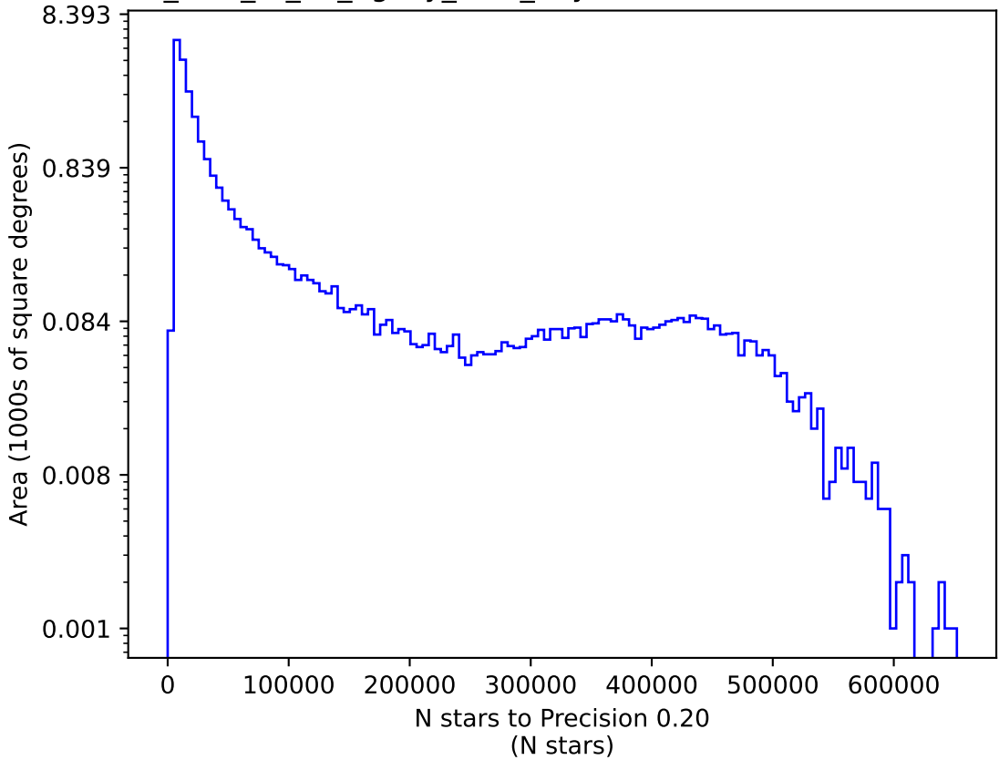
too_elab_r8_d3_ugrizy_v3.4_10yrs i: N stars to Precision 0.20
