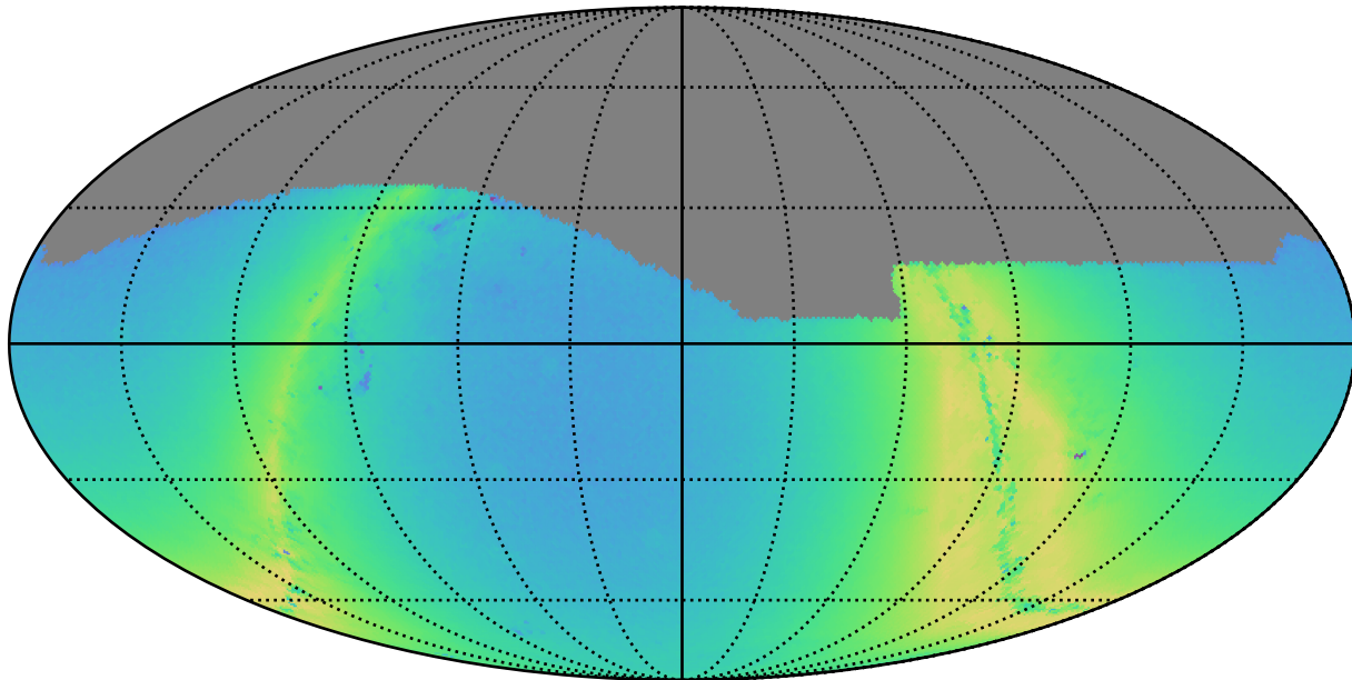
too_elab_r8_d3_ugrizy_v3.4_10yrs g: N stars to Precision 0.20
