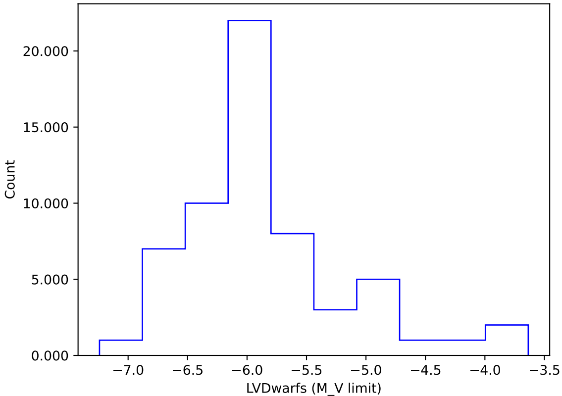
too_elab_r8_d3_ugrizy_v3.4_10yrs gi: LVDwarfs
