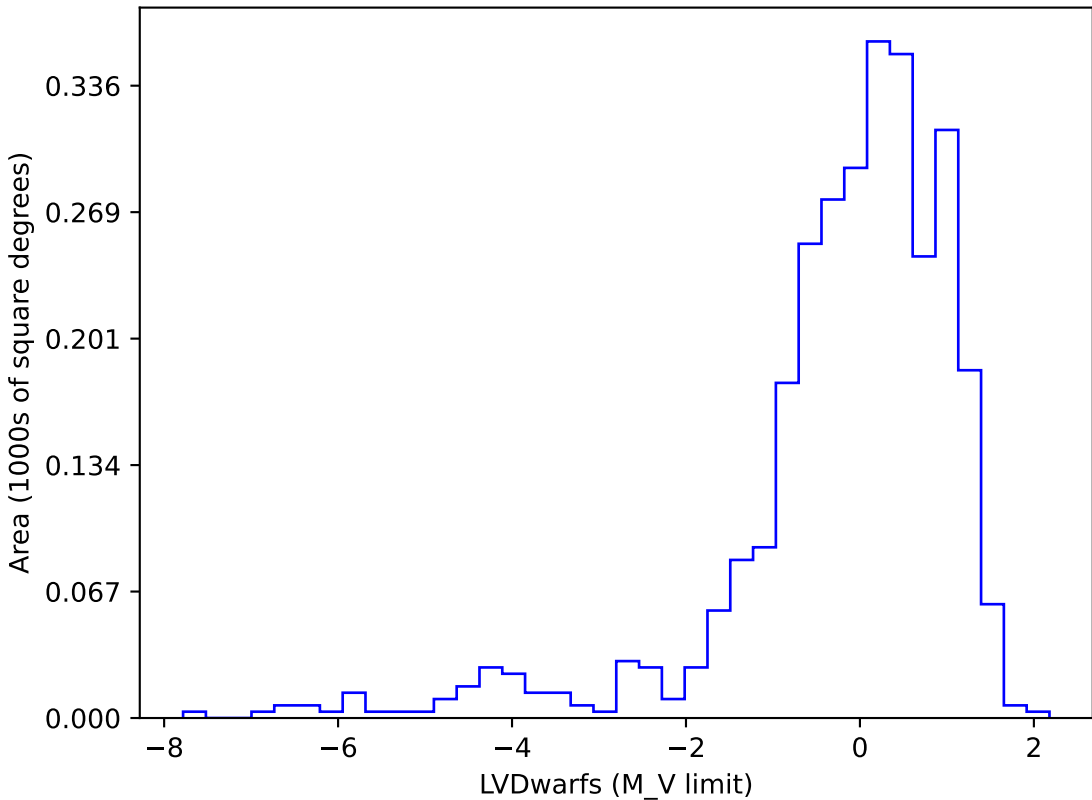
too_elab_r8_d3_ugrizy_v3.4_10yrs gi SCP: LVDwarfs
