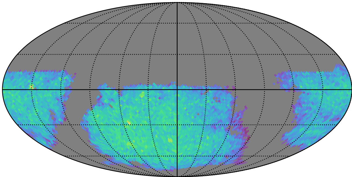
too_elab_r8_d3_ugrizy_v3.4_10yrs gi: LVDwarfs
