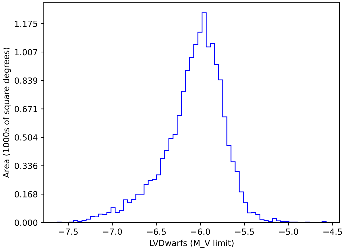
too_elab_r8_d3_ugrizy_v3.4_10yrs gi: LVDwarfs
