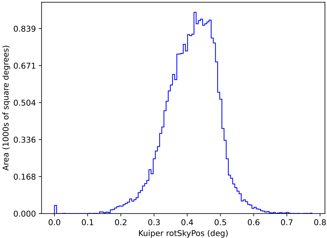
too_elab_r8_d3_ugrizy_v3.4_10yrs y: Kuiper rotSkyPos
