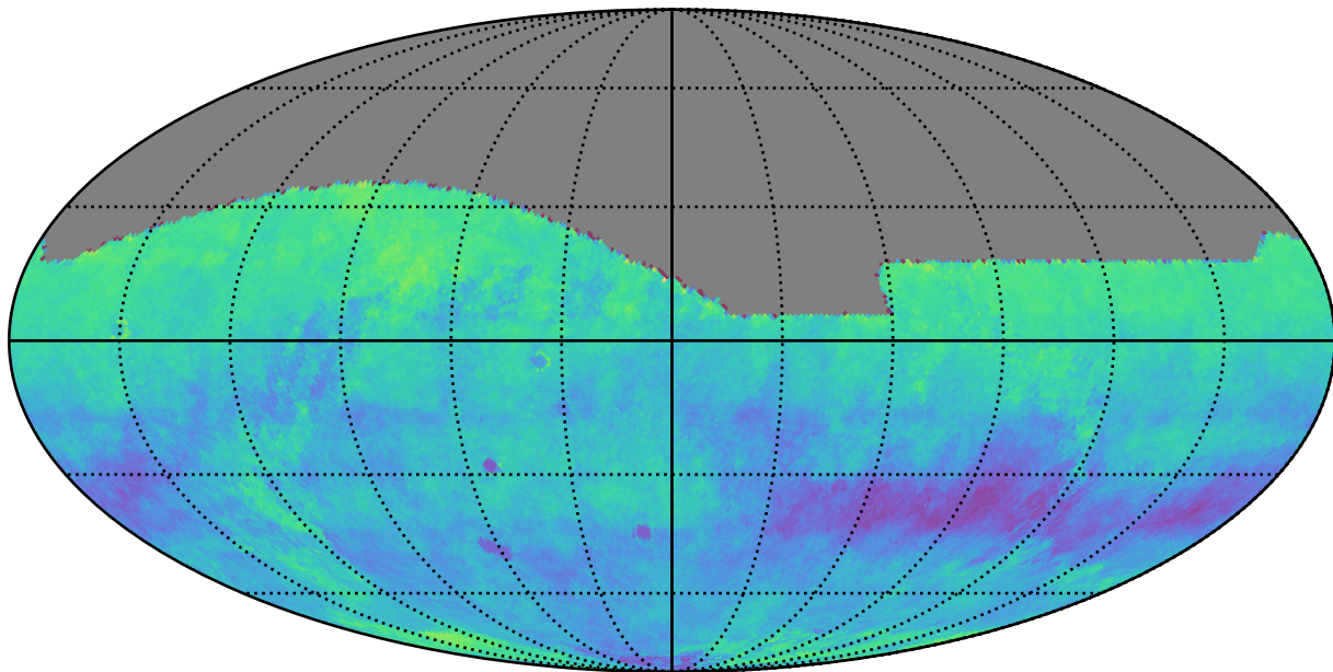
too_elab_r8_d3_ugrizy_v3.4_10yrs r: Kuiper rotSkyPos
