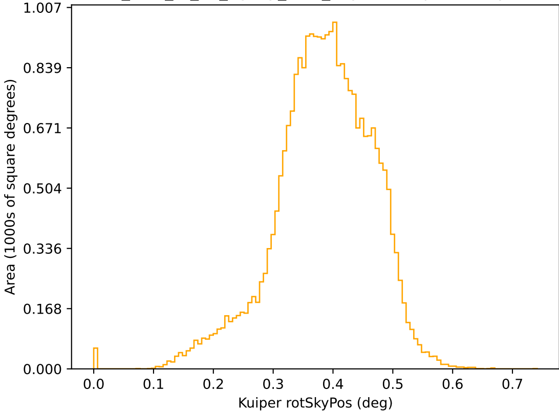
too_elab_r8_d3_ugrizy_v3.4_10yrs r: Kuiper rotSkyPos
