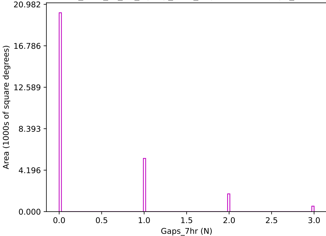
too_elab_r8_d3_ugrizy_v3.4_10yrs z band: Gaps_7hr
