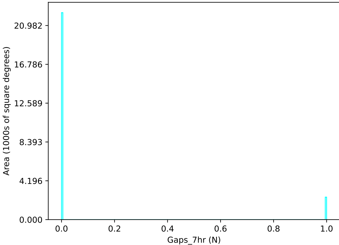
too_elab_r8_d3_ugrizy_v3.4_10yrs u band: Gaps_7hr
