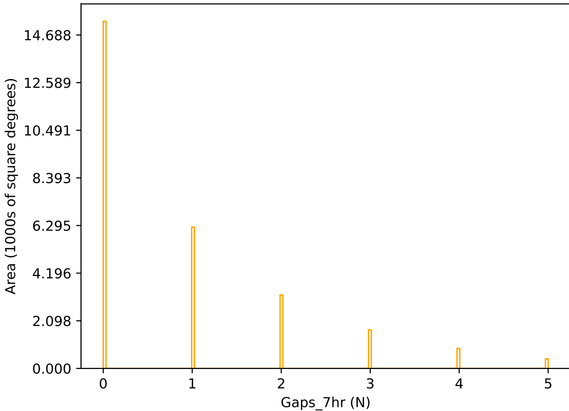
too_elab_r8_d3_ugrizy_v3.4_10yrs r band: Gaps_7hr
