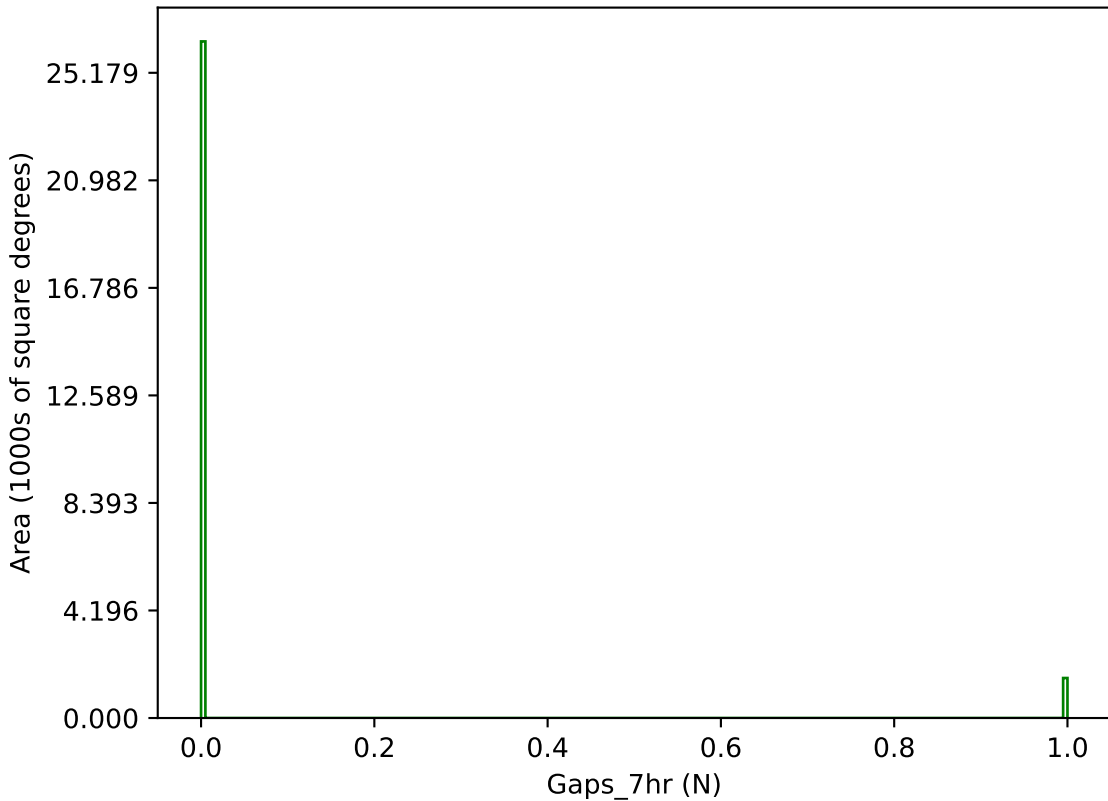
too_elab_r8_d3_ugrizy_v3.4_10yrs g band: Gaps_7hr
