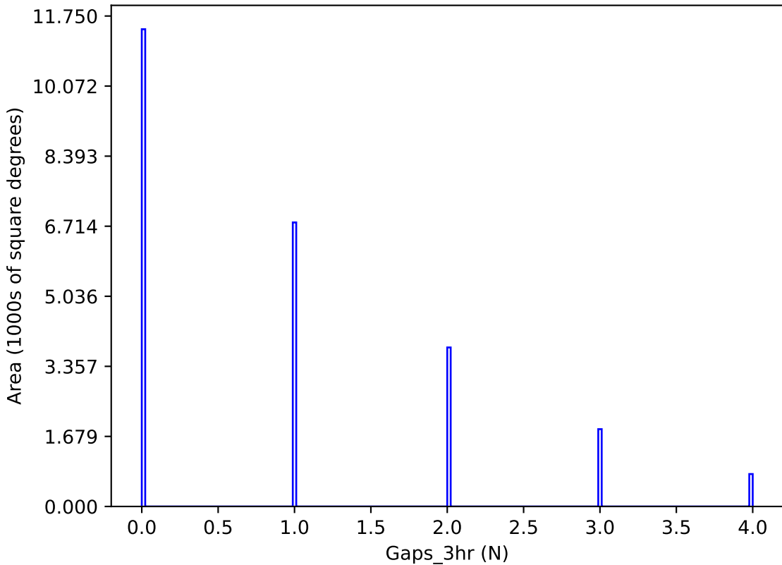
too_elab_r8_d3_ugrizy_v3.4_10yrs y band: Gaps_3hr
