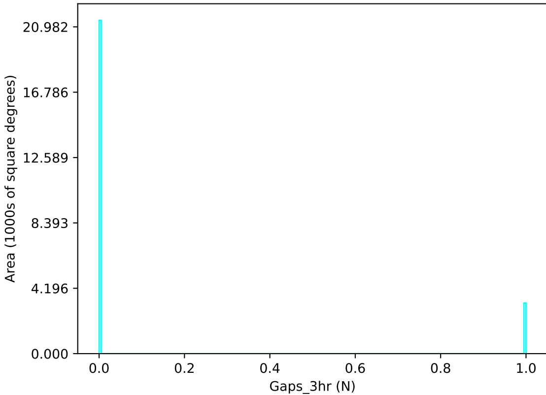
too_elab_r8_d3_ugrizy_v3.4_10yrs u band: Gaps_3hr
