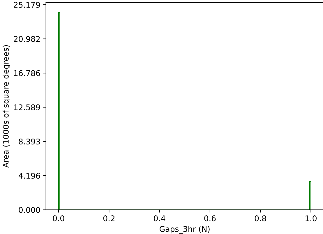
too_elab_r8_d3_ugrizy_v3.4_10yrs g band: Gaps_3hr
