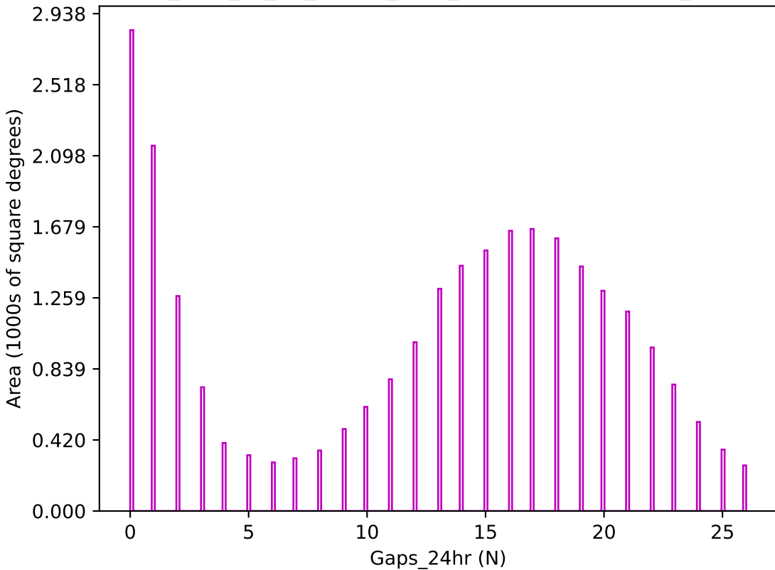
too_elab_r8_d3_ugrizy_v3.4_10yrs z band: Gaps_24hr
