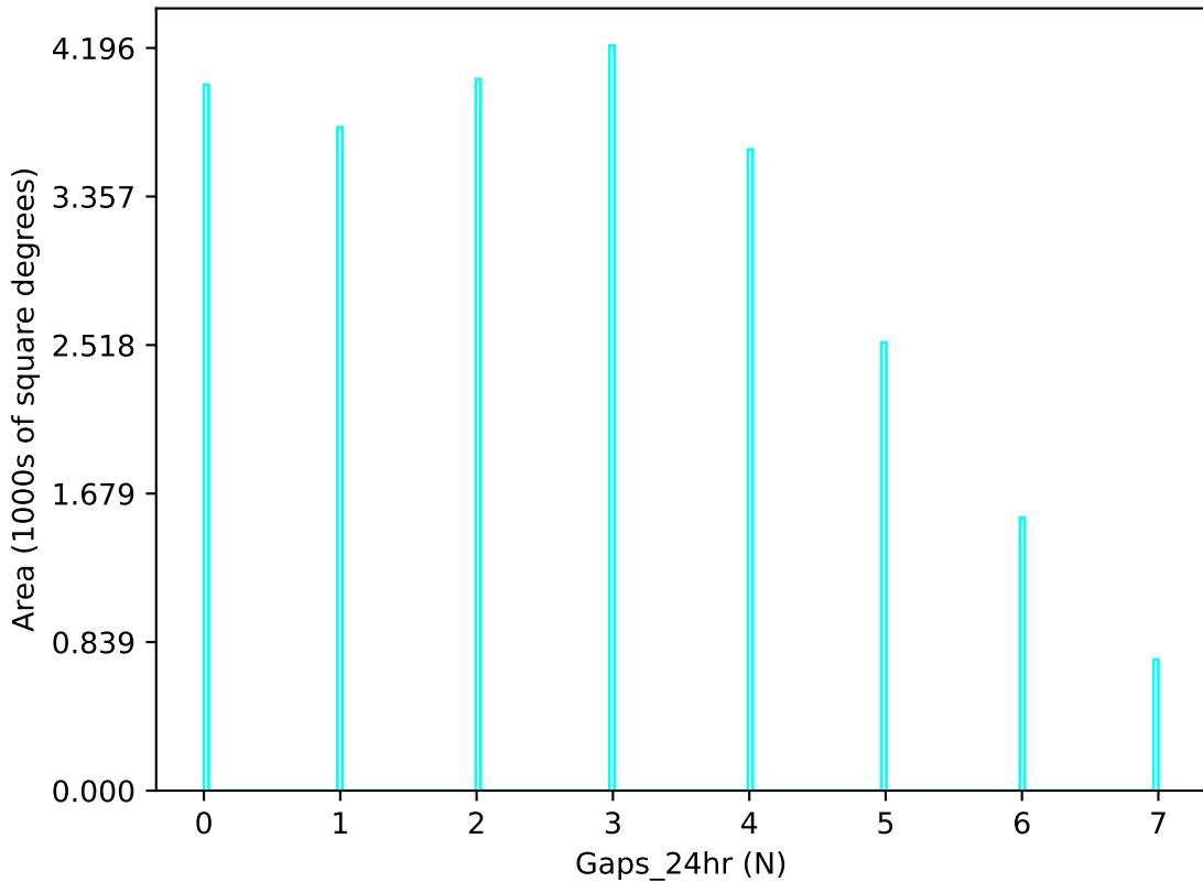
too_elab_r8_d3_ugrizy_v3.4_10yrs u band: Gaps_24hr
