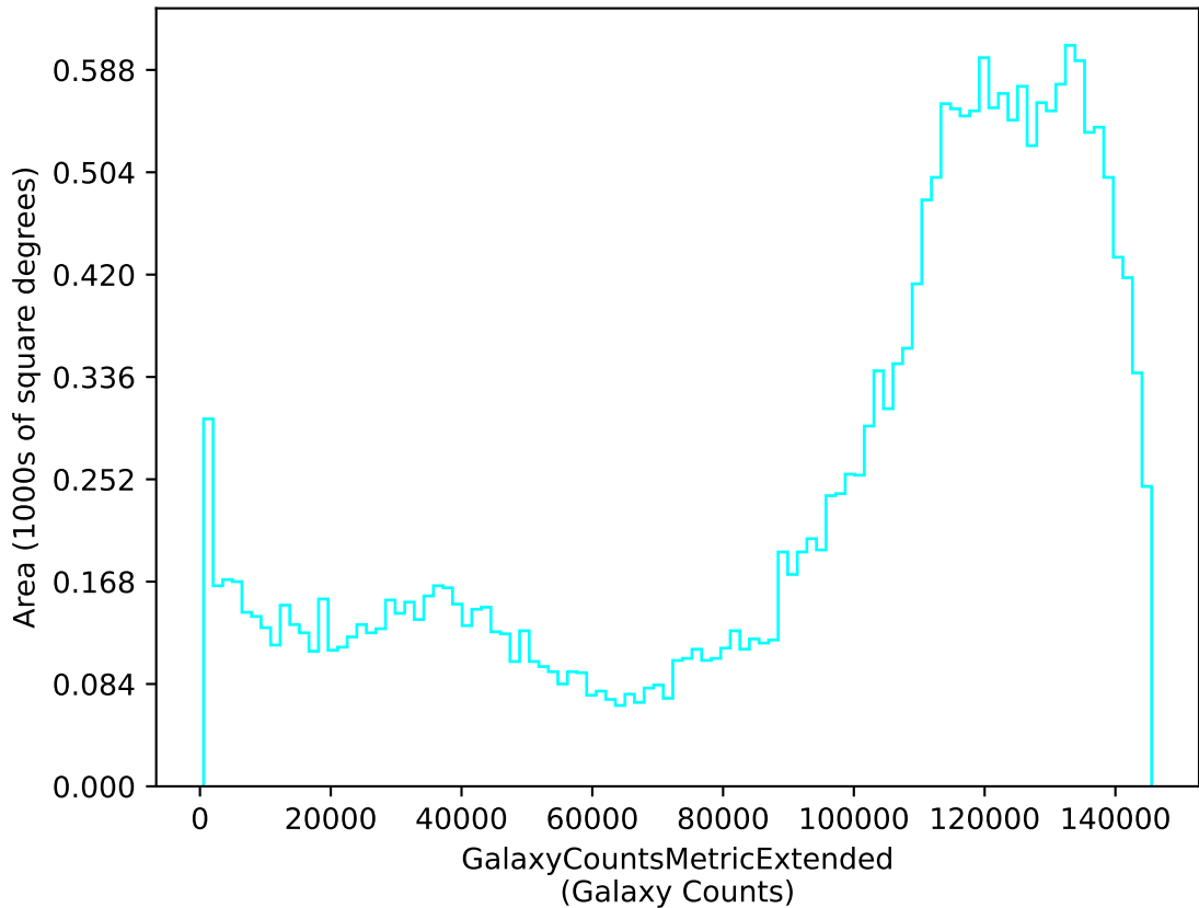
too_elab_r8_d3_ugrizy_v3.4_10yrs u: GalaxyCountsMetricExtended
