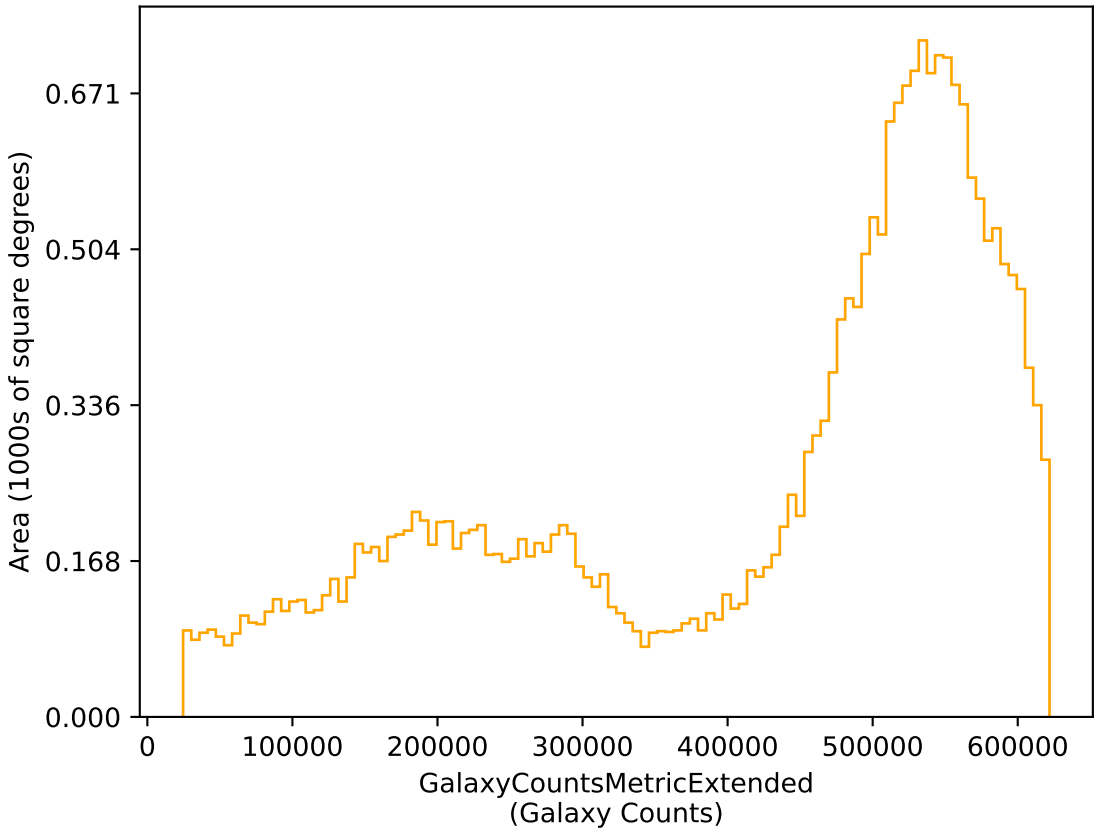
too_elab_r8_d3_ugrizy_v3.4_10yrs r: GalaxyCountsMetricExtended
