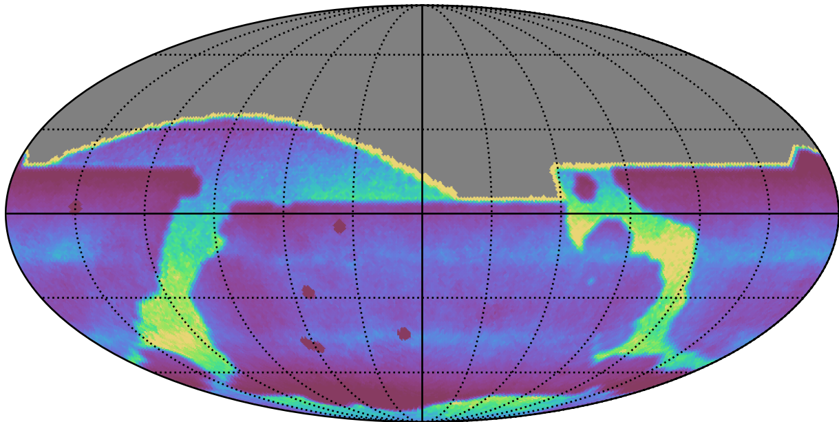
too_elab_r8_d3_ugrizy_v3.4_10yrs : DCRprecision
