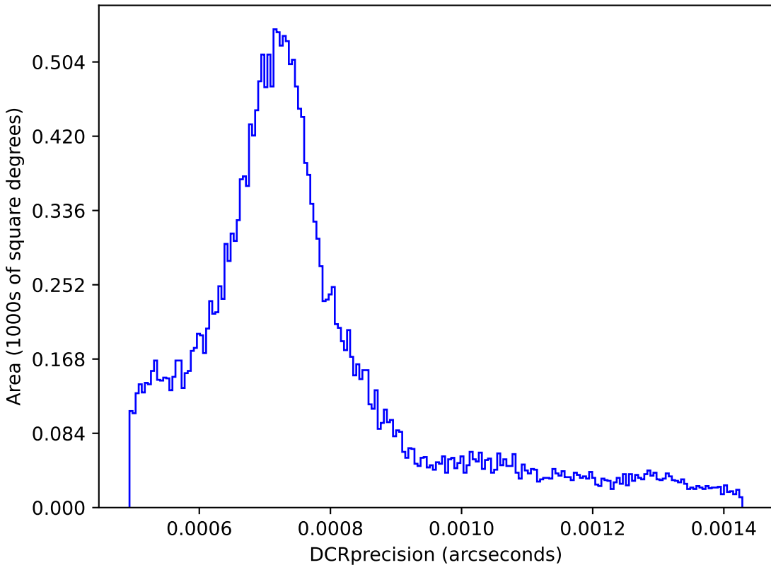
too_elab_r8_d3_ugrizy_v3.4_10yrs : DCRprecision
