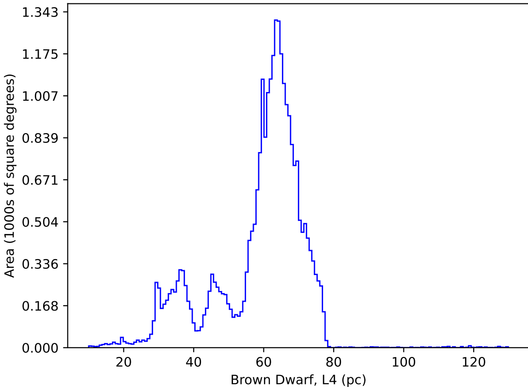
too_elab_r8_d3_ugrizy_v3.4_10yrs : Brown Dwarf, L4
