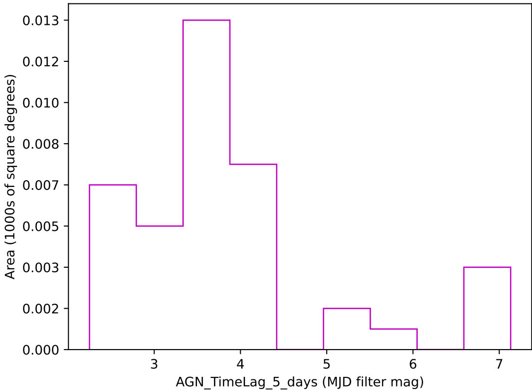
too_elab_r8_d3_ugrizy_v3.4_10yrs z band: AGN_TimeLag_5_days
