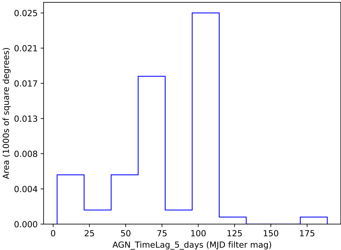
too_elab_r8_d3_ugrizy_v3.4_10yrs y band: AGN_TimeLag_5_days
