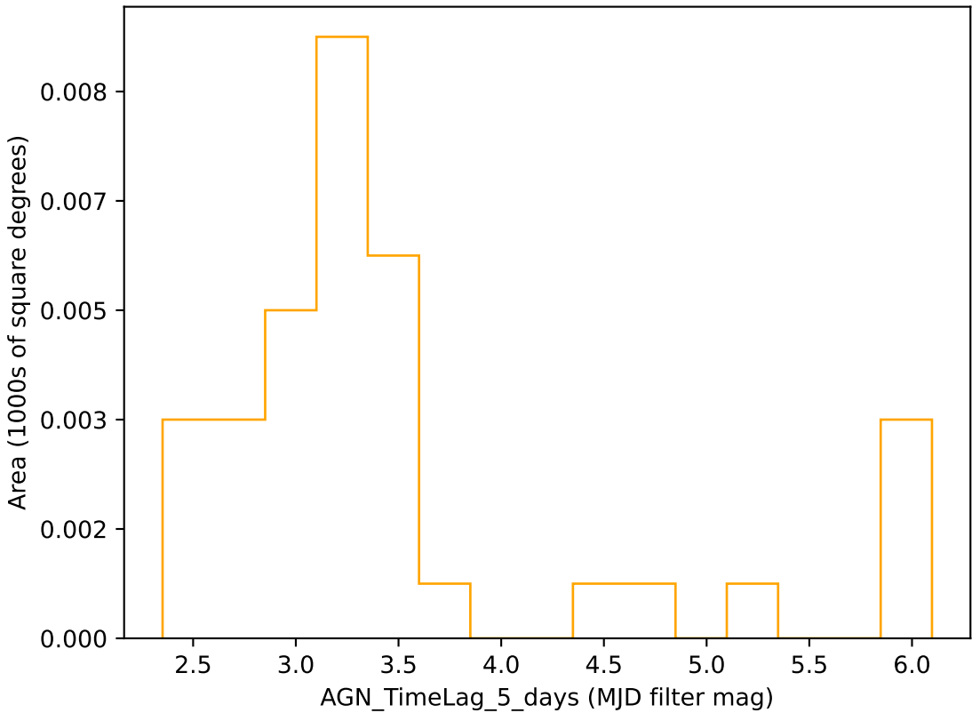
too_elab_r8_d3_ugrizy_v3.4_10yrs r band: AGN_TimeLag_5_days
