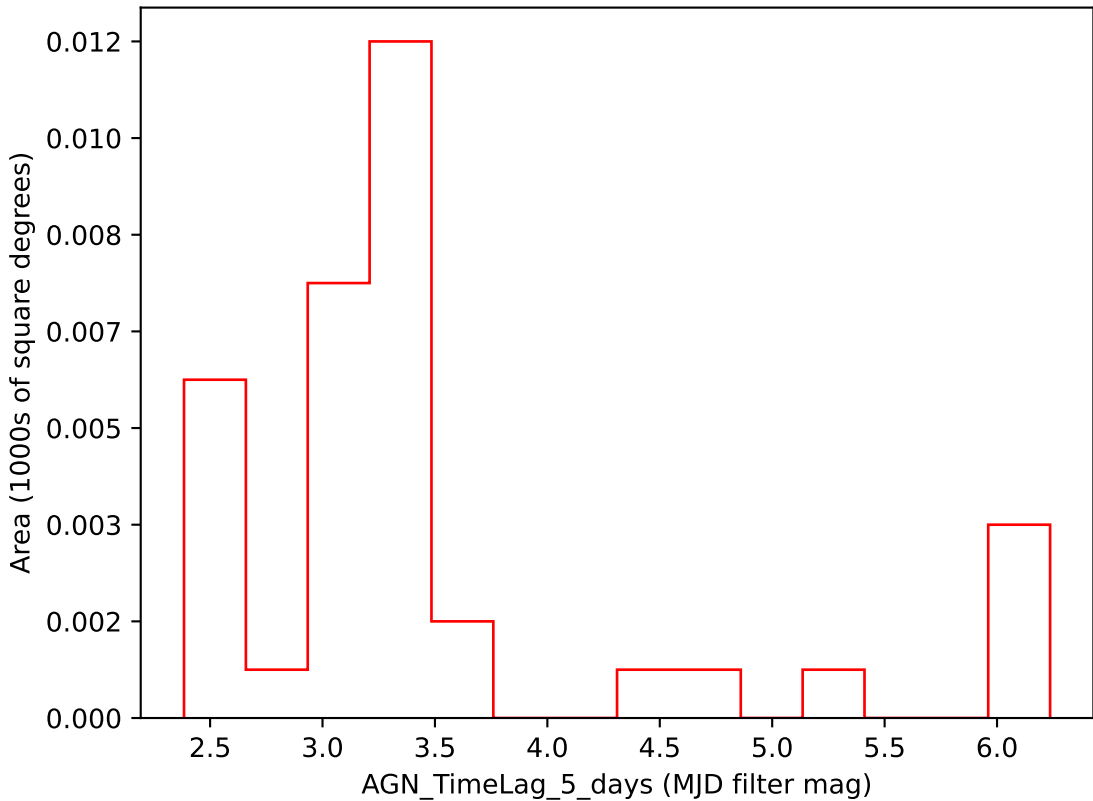
too_elab_r8_d3_ugrizy_v3.4_10yrs i band: AGN_TimeLag_5_days
