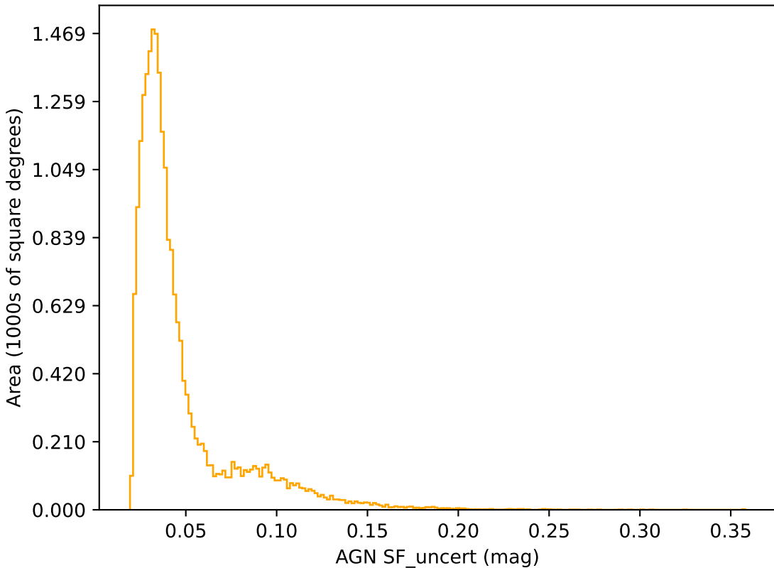
too_elab_r8_d3_ugrizy_v3.4_10yrs r band: AGN SF_uncert
