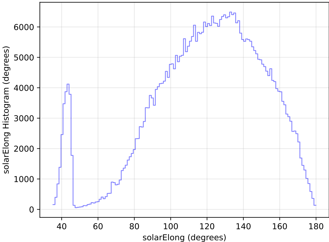
too_elab_r8_d3_ugrizy_v3.4_10yrs WFD z band: solarElong Histogram
