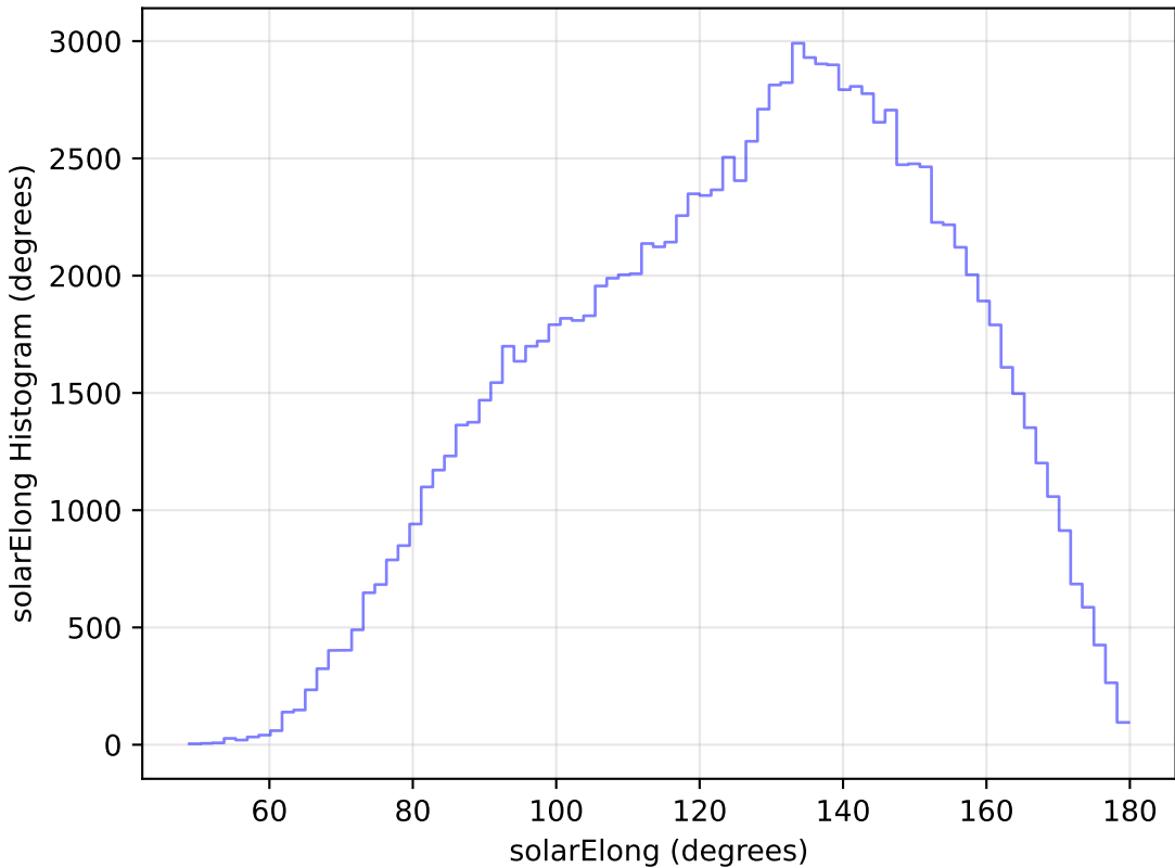
too_elab_r8_d3_ugrizy_v3.4_10yrs WFD u band: solarElong Histogram
