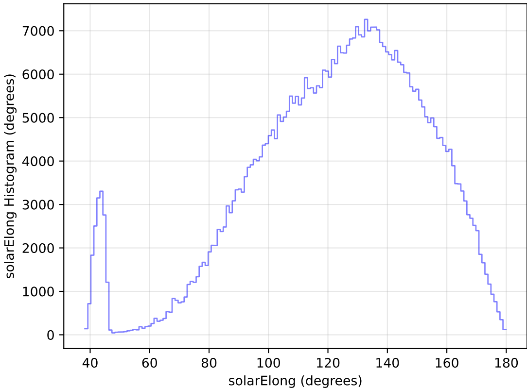
too_elab_r8_d3_ugrizy_v3.4_10yrs WFD r band: solarElong Histogram
