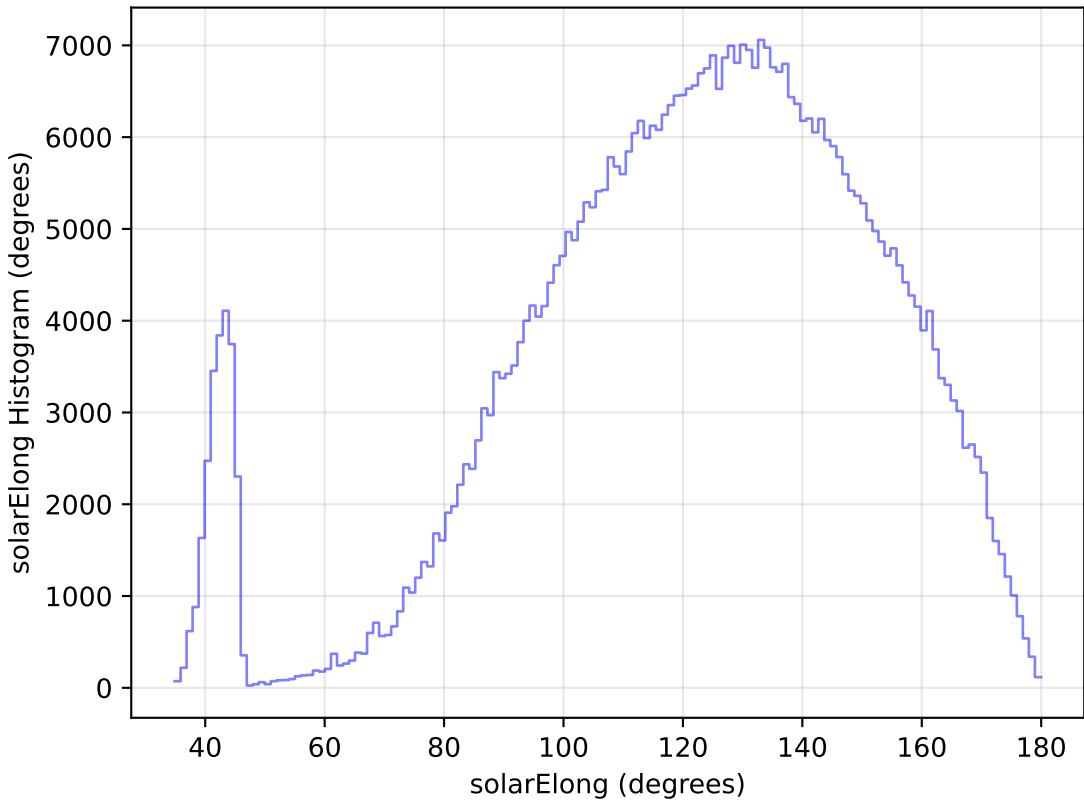
too_elab_r8_d3_ugrizy_v3.4_10yrs WFD i band: solarElong Histogram
