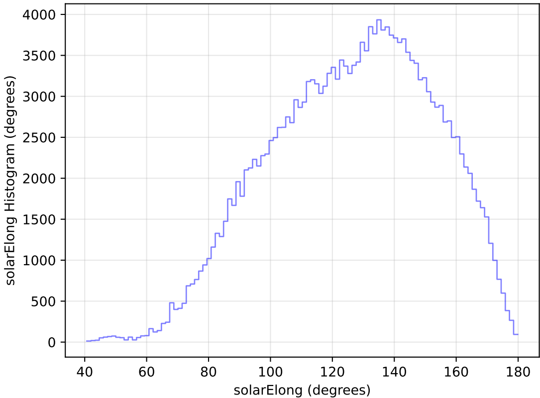
too_elab_r8_d3_ugrizy_v3.4_10yrs WFD g band: solarElong Histogram
