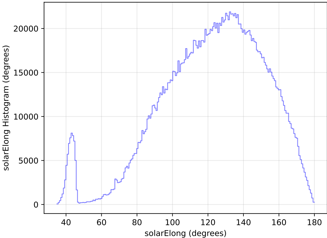
too_elab_r8_d3_ugrizy_v3.4_10yrs WFD all bands: solarElong Histogram
