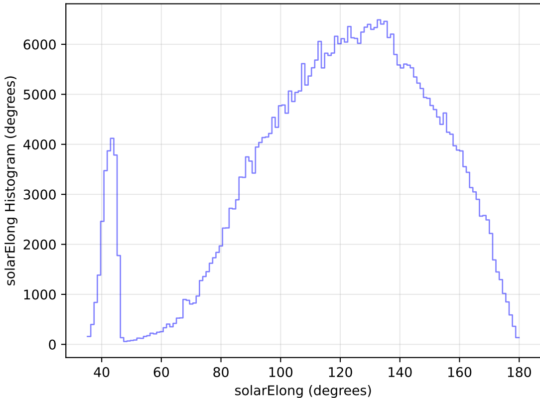
too_elab_r8_d3_ugrizy_v3.4_10yrs All sky z band: solarElong Histogram
