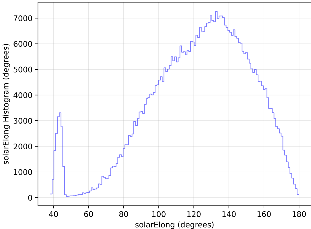
too_elab_r8_d3_ugrizy_v3.4_10yrs All sky r band: solarElong Histogram
