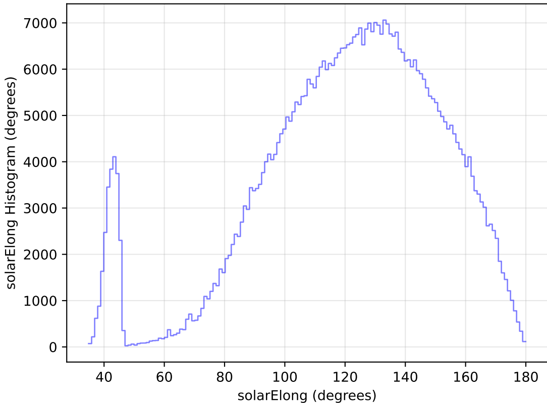
too_elab_r8_d3_ugrizy_v3.4_10yrs All sky i band: solarElong Histogram
