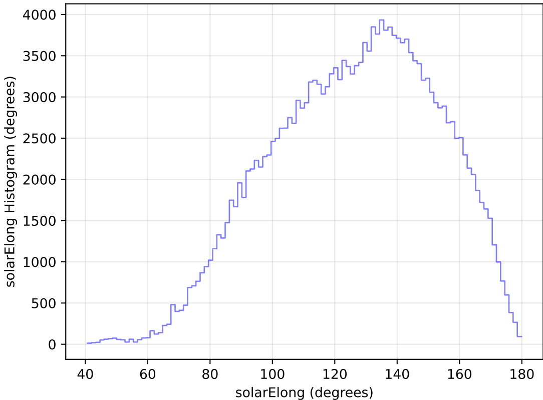
too_elab_r8_d3_ugrizy_v3.4_10yrs All sky g band: solarElong Histogram
