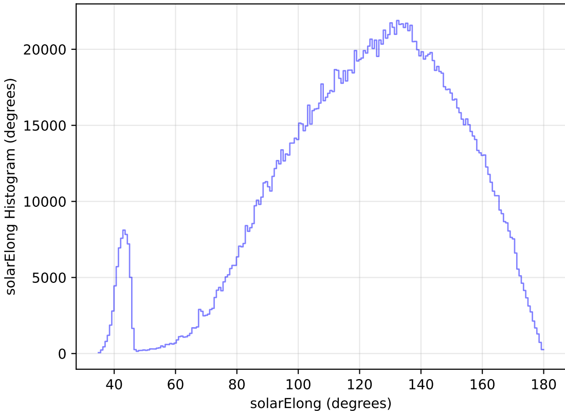
too_elab_r8_d3_ugrizy_v3.4_10yrs All sky all bands: solarElong Histogram
